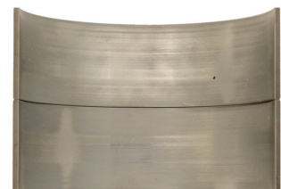
Pleuellager
